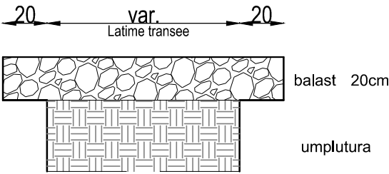
Acostament
