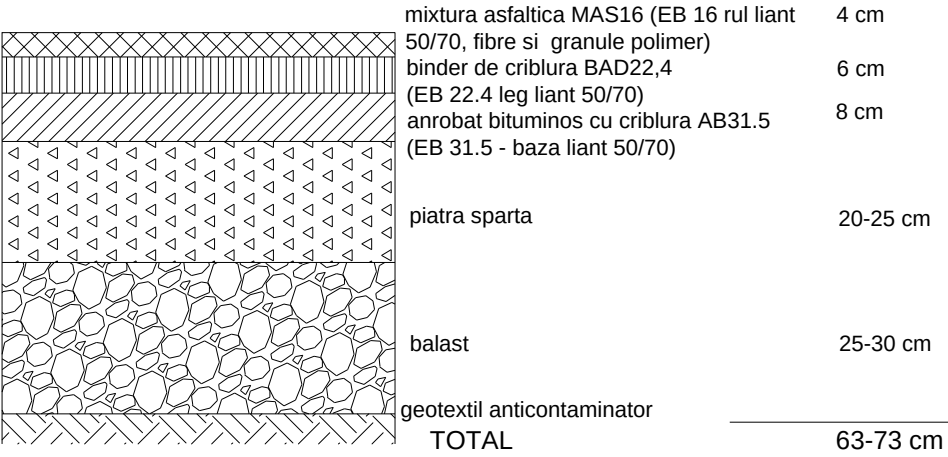
Drum asfalt
