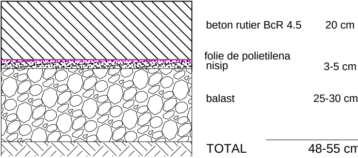
Drum beton
