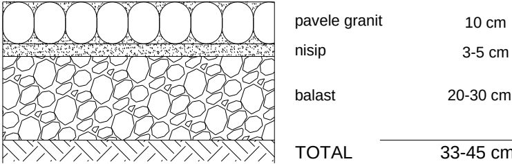
Drum pavele granit
